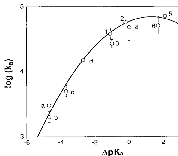
FIGURE 2 Dependence of the logarithm of k_B ( \text{s}^{-1} ) on \Delta\text{pK}_a (the \text{pK}_a of the donor group subtracted from the \text{pK}_a of the zinc-bound water). k_B is the rate constant for donation of protons to the zinc-bound hydroxide accompanying the dehydration of \text{HCO}_3^- obtained from ^{18}\text{O} exchange experiments. The entries are wild type and mutants of HCA III listed in Table 1. The solid line is a least-squares fit of the Marcus equation (Eq. 6) to the entries of Table 1 (a–d, 1–6) giving \Delta G_0^\ddagger = 2.2 \pm 0.5 \text{ kcal/mol} , with work functions w^r = 10.8 \pm 0.1 \text{ kcal/mol} and w^p = 4.0 \pm 1.6 \text{ kcal/mol} .
